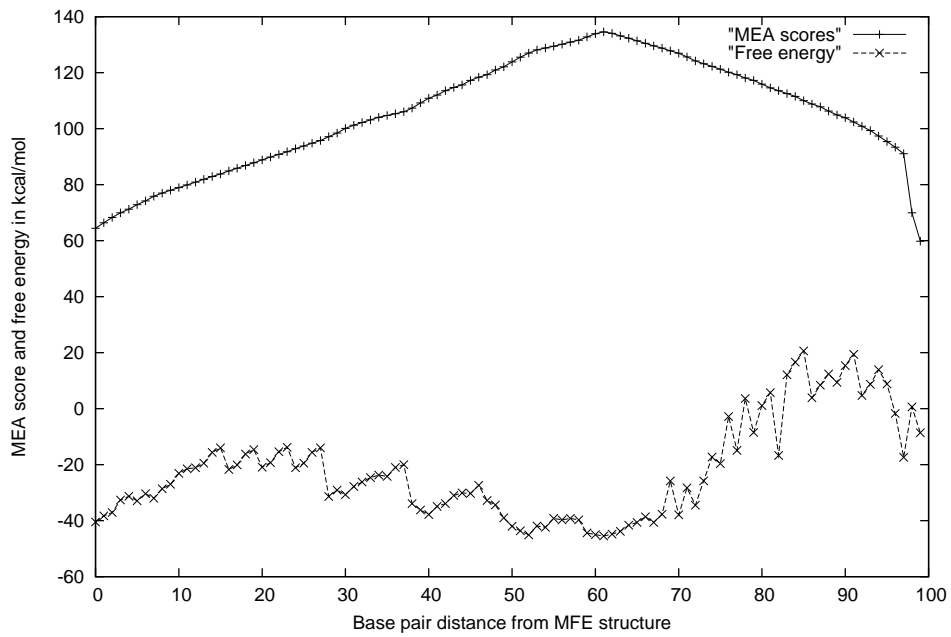
TPP-riboswitch, AF269819/1811-1669
