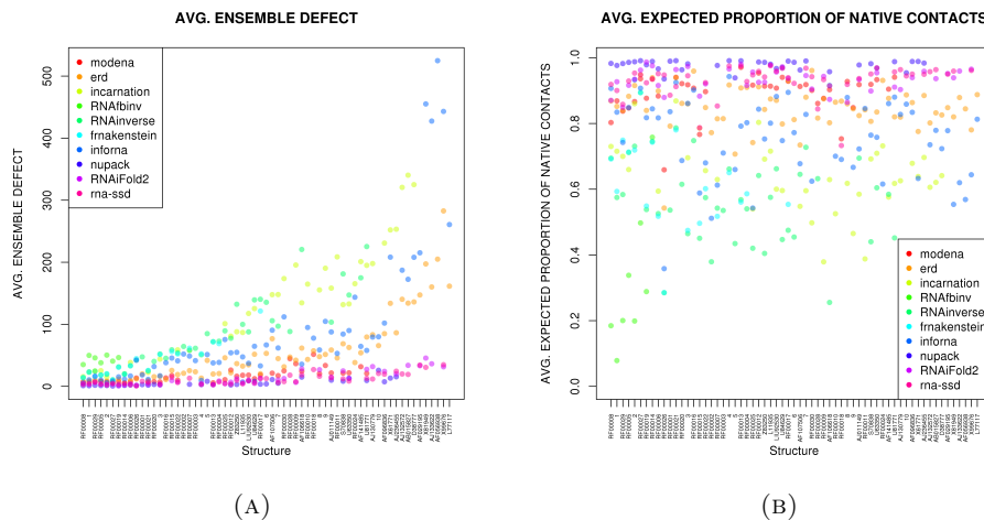
FIGURE 3. (a) Average ensemble defect for inverse folding software, where the (non length-normalized) averages are taken over all sequences returned for a fixed target structure. Name of the target structure is given on the x -axis, arranged in increasing length (length is not drawn to scale); y -axis depicts the average ensemble defect for the output of each software, on each target. (b) Average proportion of native (target) contacts, where the (non length-normalized) averages are taken over all sequences returned for a fixed target structure. Name of the target structure is given on the x -axis, arranged in increasing length (length is not drawn to scale); y -axis depicts the expected proportion of base pairs in the target structure that are present in the low energy ensemble of all structures, for each target. Benchmarking data, both raw data and length-normalized data, as well as scatter plots for for all measures can be found at the RNAiFold 2.0 web site in the ‘Download’ tab.
