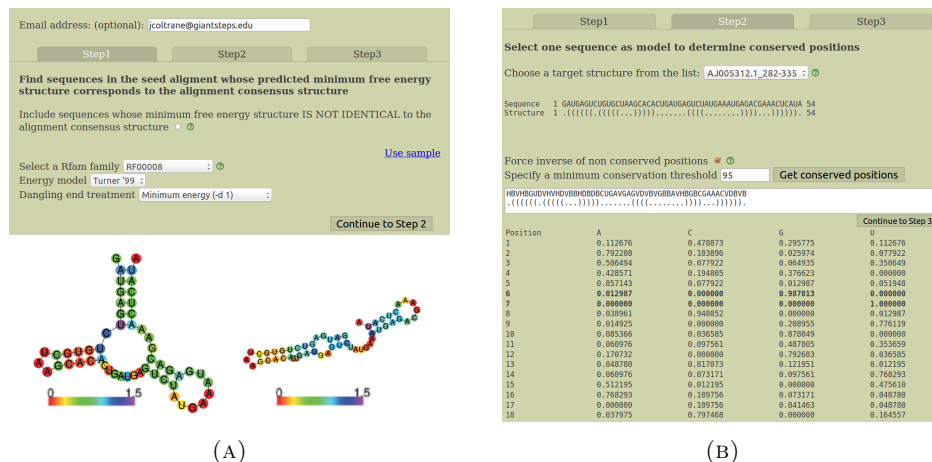
FIGURE 1. (a) First of 3 screens in RNA Rfam-based Design , invoked to automate the generation of synthetic RNAs likely to adopt the same function as RNAs in a user-specified Rfam class. Computations may take long, so though optional, it is advisable to enter an email address to be informed of the results when ready. The user must select an Rfam family and the energy model, i.e. Turner'99 or Turner'04 [30] together with a dangle state. As shown in the figure, the Turner'99 parameters (Vienna 1.8.5) can prove to be a better choice than the Turner'04 parameters (Vienna 2.1.7) in certain circumstances – here, Vienna 1.8.5 predicts the correct, functional structure for the hammerhead type III ribozyme (left image) from Peach Latent Mosaic Viroid (PLMVd) with accession code AJ005312.1/282-335, while the Vienna 2.1.7 predicts the incorrect structure (right image). (b) Second of 3 screens in RNA Rfam-based Design , where the user selects a sequence in the pull-down menu; this sequence, which belongs to the chosen Rfam family will serve as an initial model to generate synthetic sequences. Each displayed sequence folds into the Rfam consensus structure when using the selected energy parameters (if no sequence is shown, then no sequence has this property). In this screen, the user may specify that RNAiFold 2.0 automatically generate sequence constraints for positions that are conserved in the Rfam seed alignment to user-specified minimum threshold; to avoid generating solutions that are too similar to the model sequence, the server automatically generates IUPAC constraints to disagree with the model sequence at all positions where the seed alignment has less than the specified conservation threshold. The position-specific compositional frequency (profile) of the Rfam seed alignment is displayed for each position.
