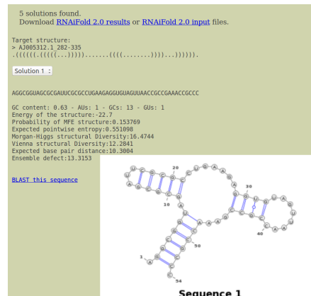
FIGURE 2. (a) Third of 3 screens in Rfam-based Design , where the user can enter additional structure compatibility and incompatibility constraints, which require all solutions to be compatible with a second structure (in addition to folding into the target structure), and which do not allow base pairing at positions stipulated in the incompatibility constraints. (b) Output from the pipeline described in the three previous screen shots. Note that the GC-content, average positional entropy, ensemble defect and other structural diversity measures are computed. These measures provide an idea of how similar the low energy ensemble of structures resembles the minimum free energy structure, which is guaranteed to be identical to the user-input target structure.
