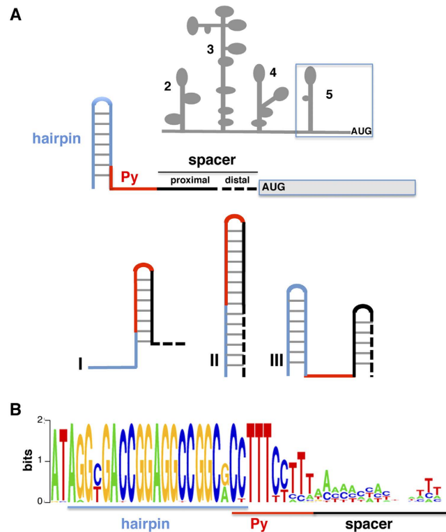
Figure 1. (A) Design strategy for synthetic RNAs harboring distinct conformations of the pyrimidine tract. (Top) Schematic representation of the FMDV IRES, organized in domains 2, 3, 4, and 5. Diagram of the structural motifs of the wild type domain 5: a hairpin (blue line), pyrimidine tract (Py) (red line) and a spacer (black line), including a proximal and a distal sequence, upstream of the functional start codon (AUG) of the reporter gene. (Bottom) Design of RNA families I, II or III. (B) The pattern of nucleotide conservation (measured in bits) of domain 5 (nts 417–462) is represented by a sequence logo obtained from the alignment of the FMDV IRES sequences of field isolates deposited in data banks.
